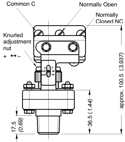
Fig. 7: Diaphragm seal piston pressure switch type E1S-...
